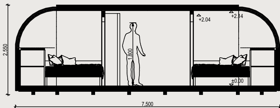
SECTION B 1:50
